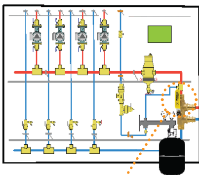
Primary / Secondary Piping Pro-Pal Loop Purge Tee OPEN
